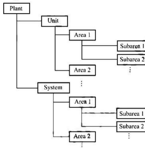
Figure 4.2.1 Plant breakdown structure
