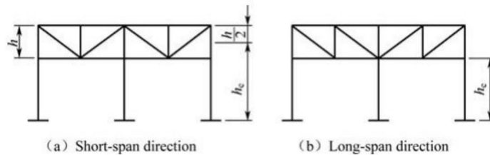
Figure 12.2.1-3 Rigid frame
